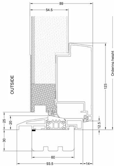
Section - bottom
